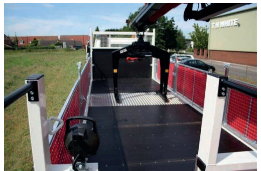
Wisa deck flooring with aluminium overlay
